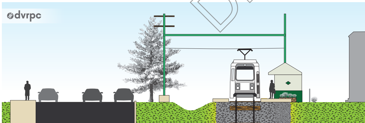
Figure 17 | Single track in exclusive right-of-way, typical cross-section
