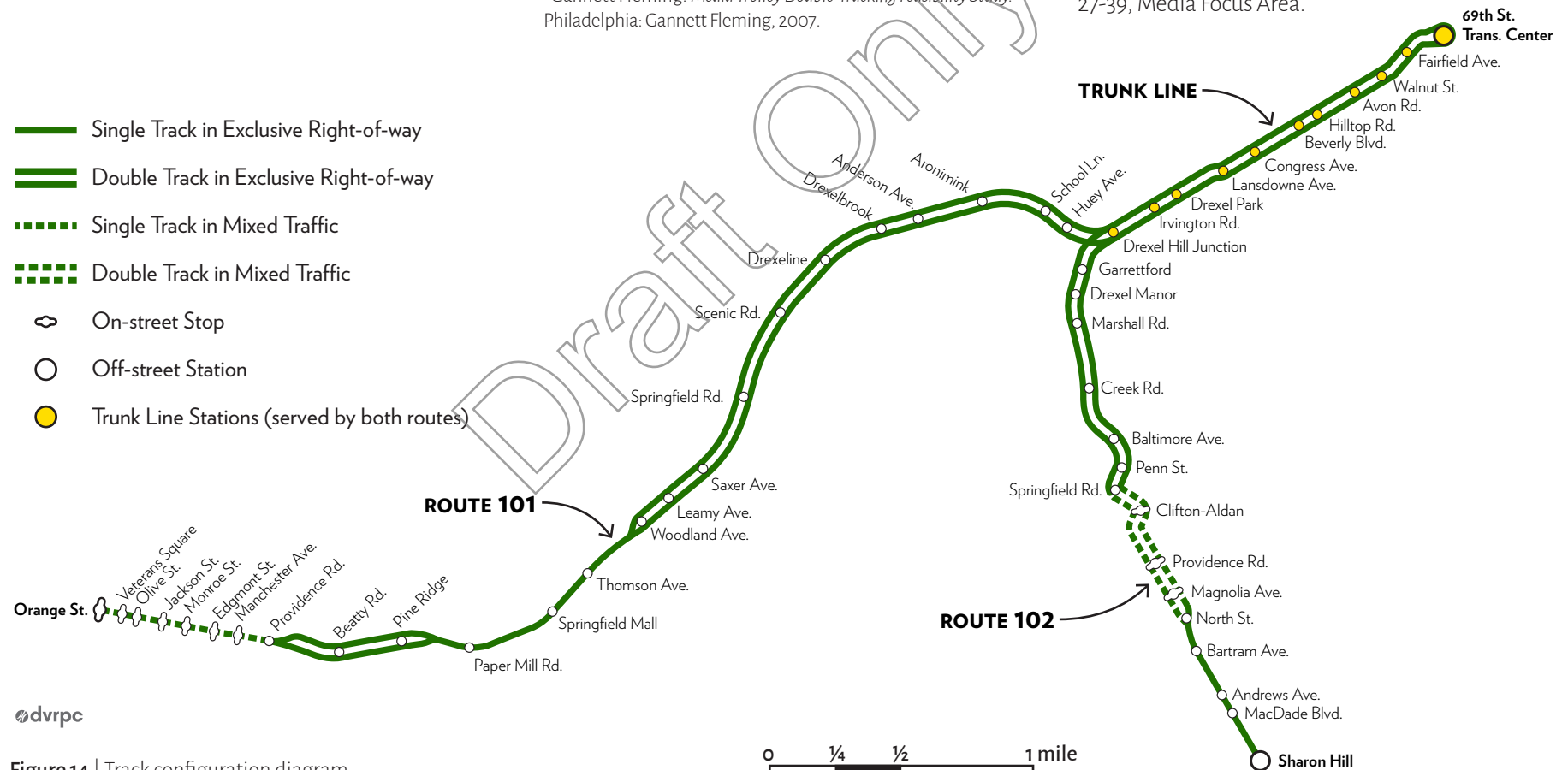
Figure 14 | Track configuration diagram
