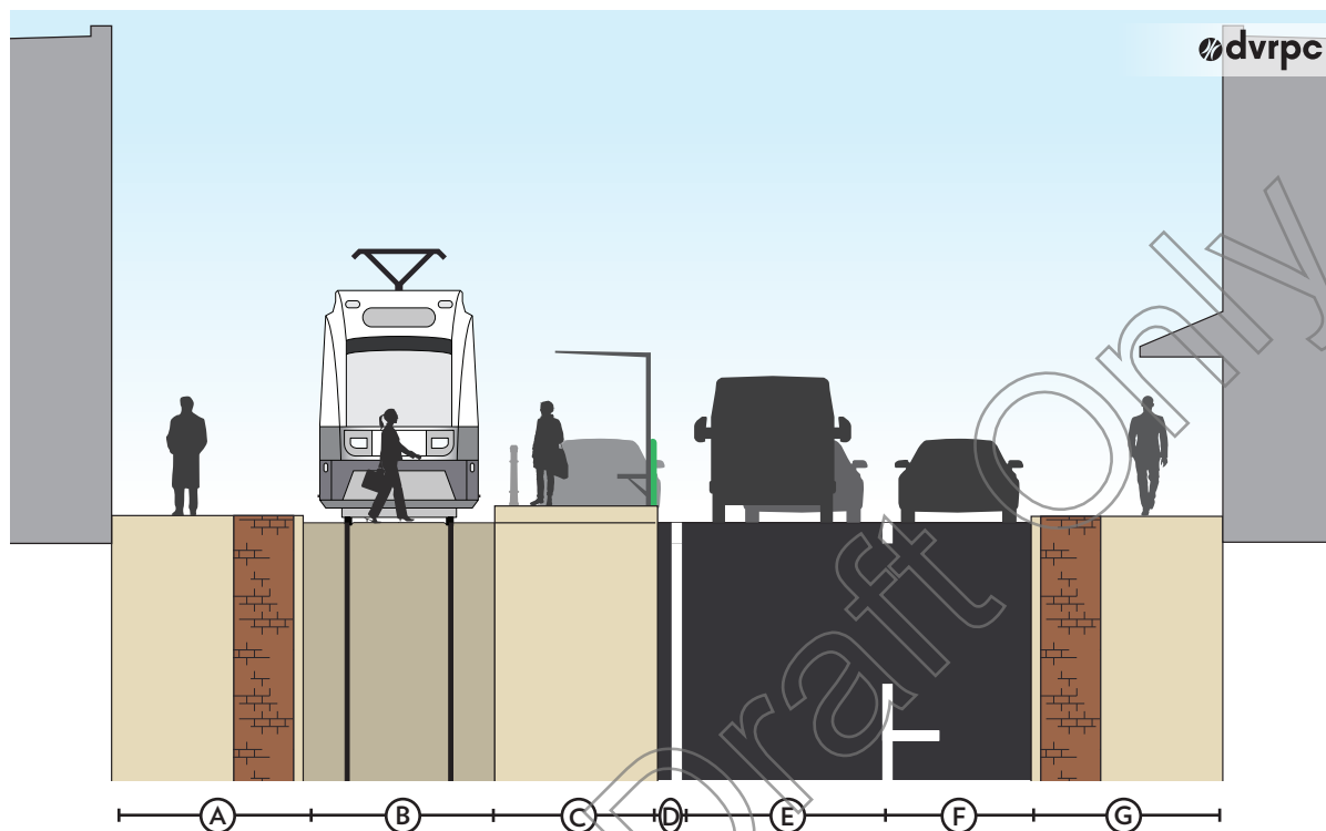
Figure 73 | One-way Street: Platform Station: Section
