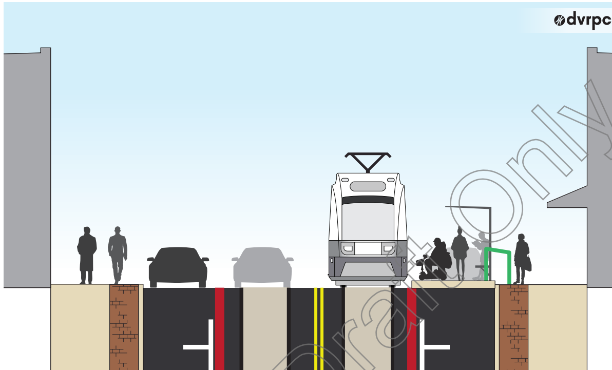
Figure 66 | Curb Extension Station: Section
