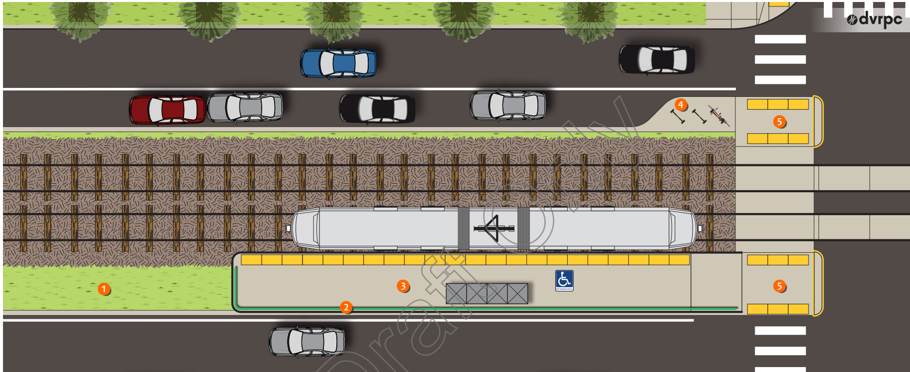
Figure 47 | Off-street Station: Plan
