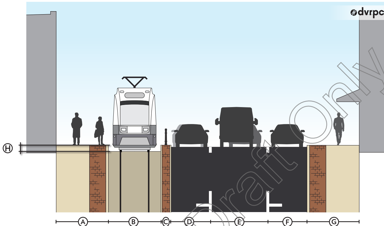
Figure 69 | One-way Street: Curbside Station: Section
