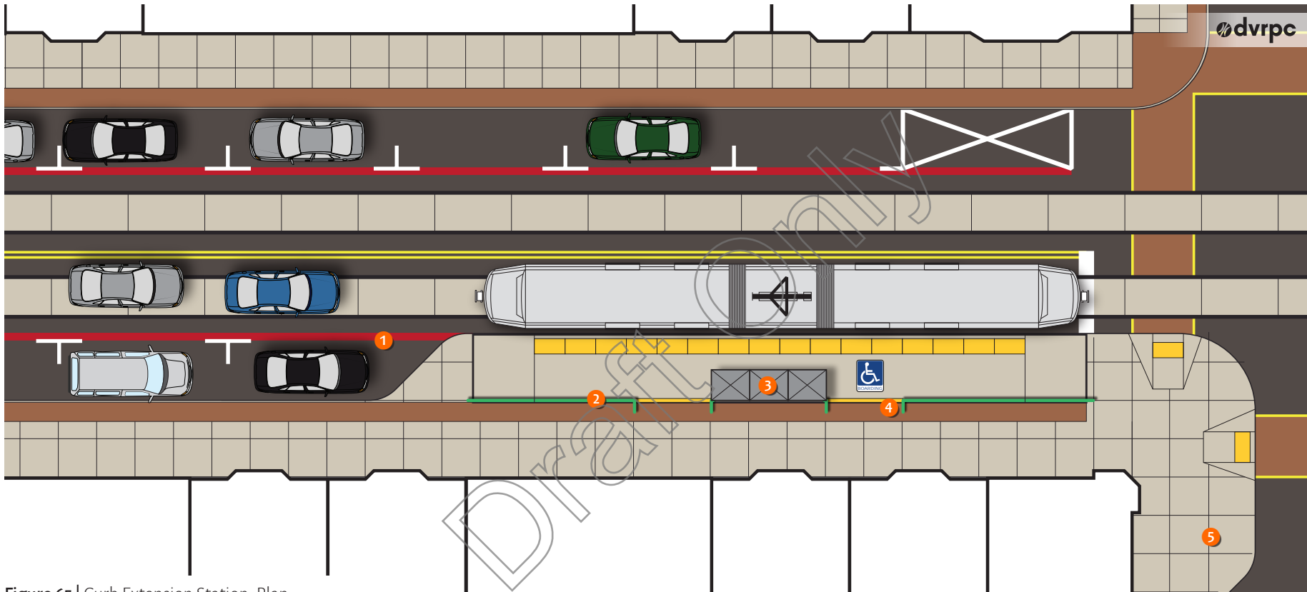
Figure 65 | Curb Extension Station: Plan
