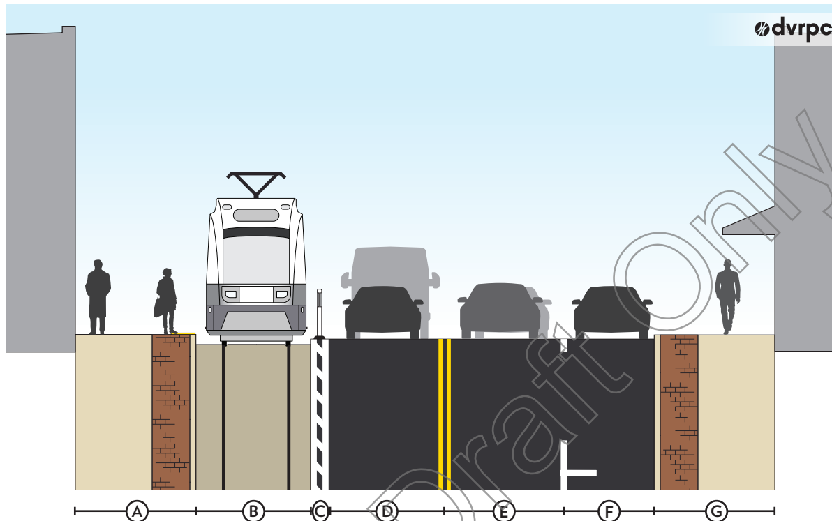
Figure 71 | Two-way Street: Curbside Station: Section (at station)
