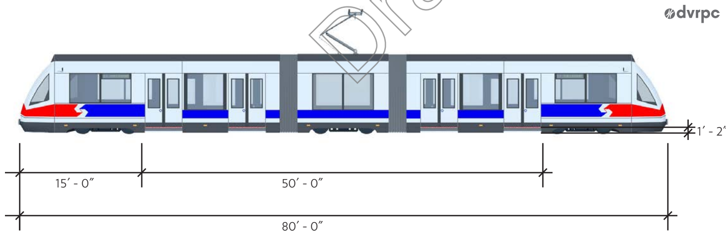
Figure 37 | Design vehicle dimensions, side elevation
