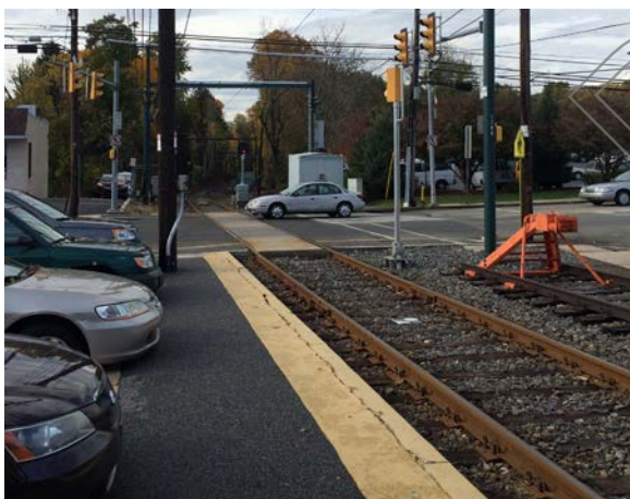
Figure 119 | Woodland Avenue, platform looking east
