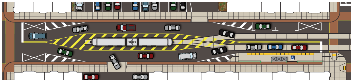
Figure 67 | Curb Extension Station: End-of-line
