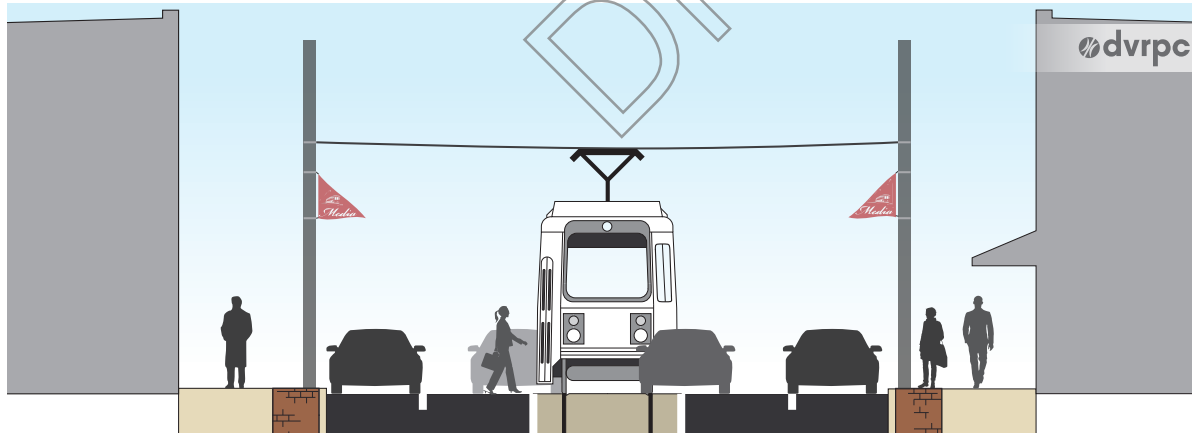
Figure 21 | Single track in mixed traffic, typical cross-section
