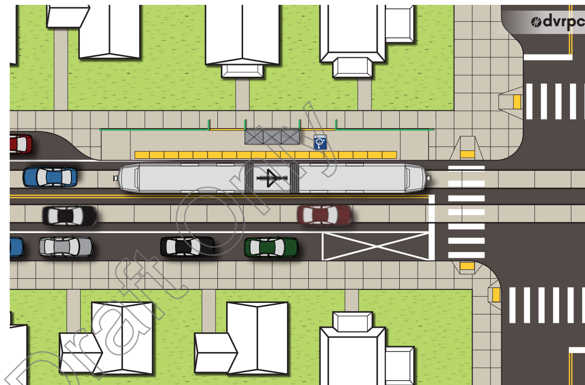
Figure 55 | Curb Extension Station: Far-side variation
