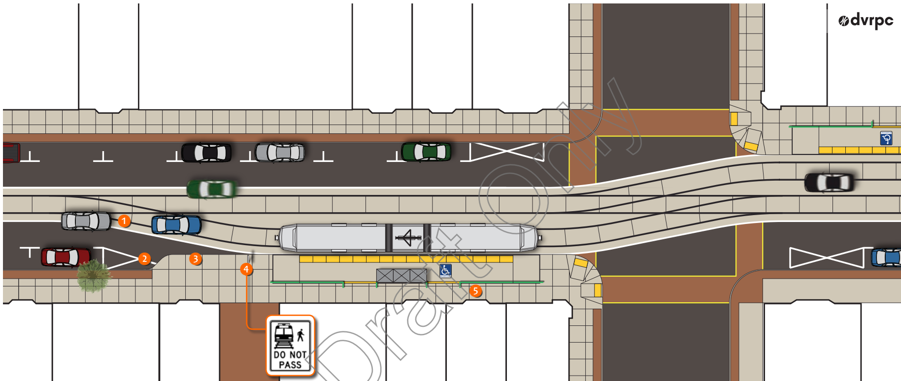
Figure 63 | Track Siding Station: Plan
