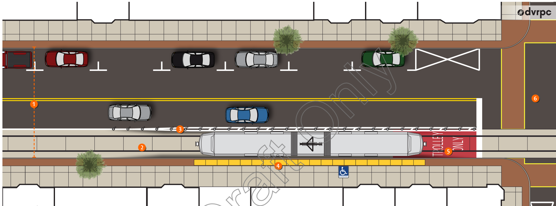
Figure 70 | Two-way Street: Curbside Station: Plan
