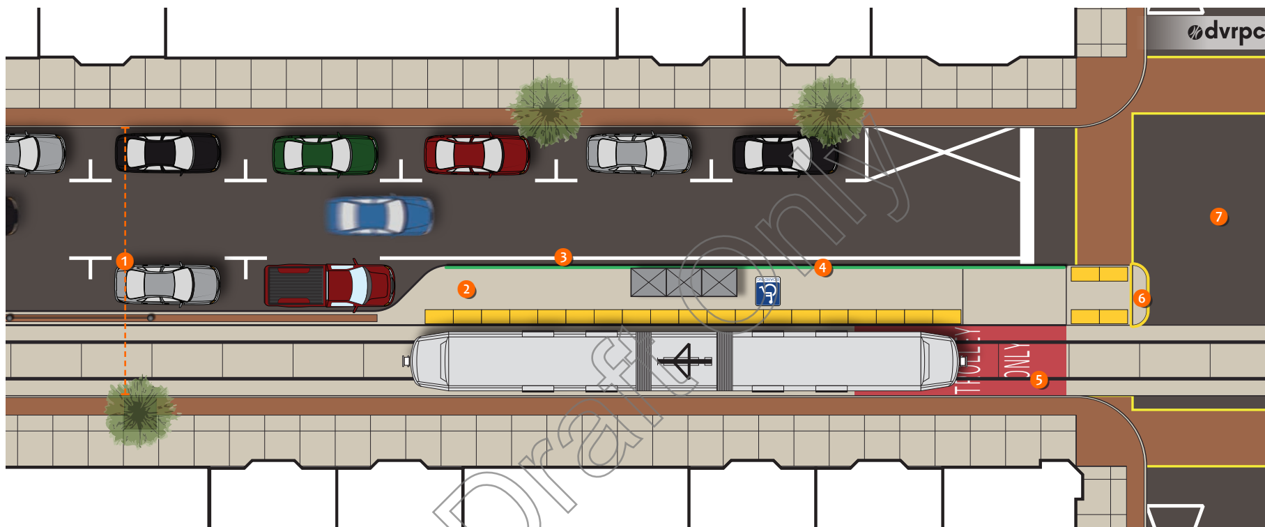
Figure 72 | One-way Street: Platform Station: Plan
