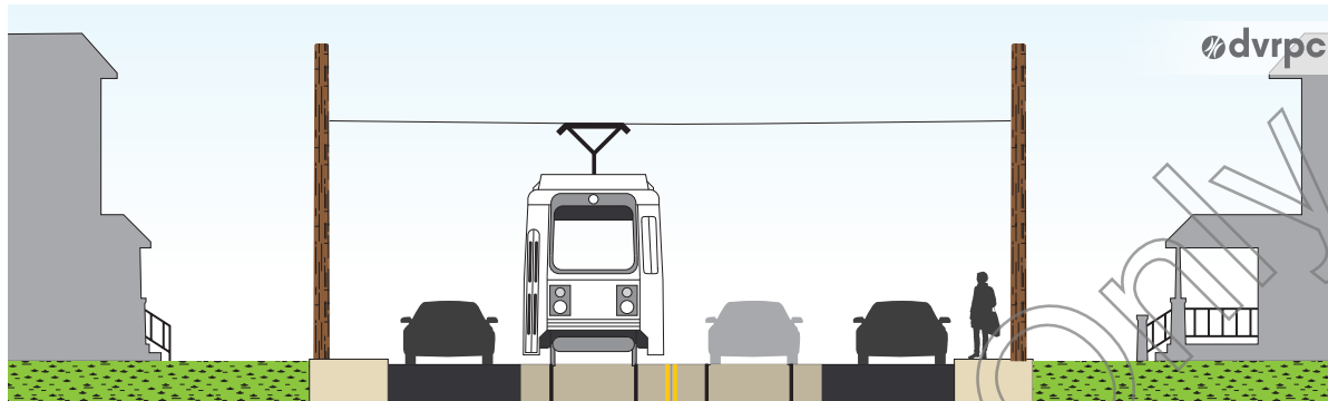
Figure 19 | Double track in mixed traffic, typical cross-section
