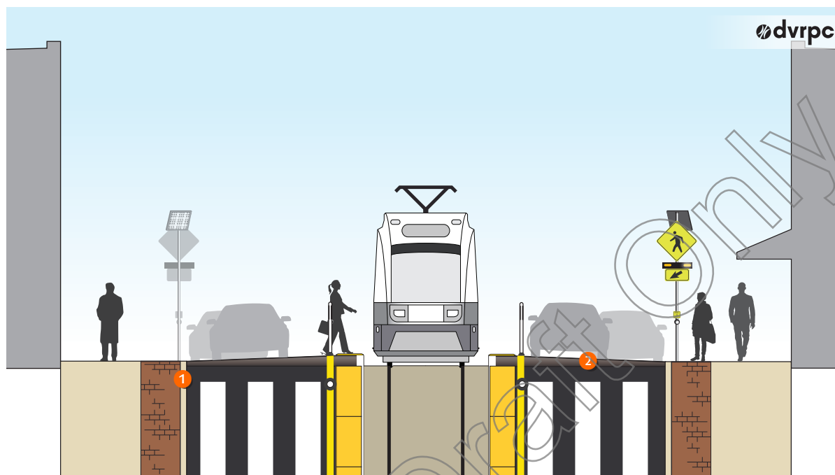
Figure 62 | Speed Table Station: Section
