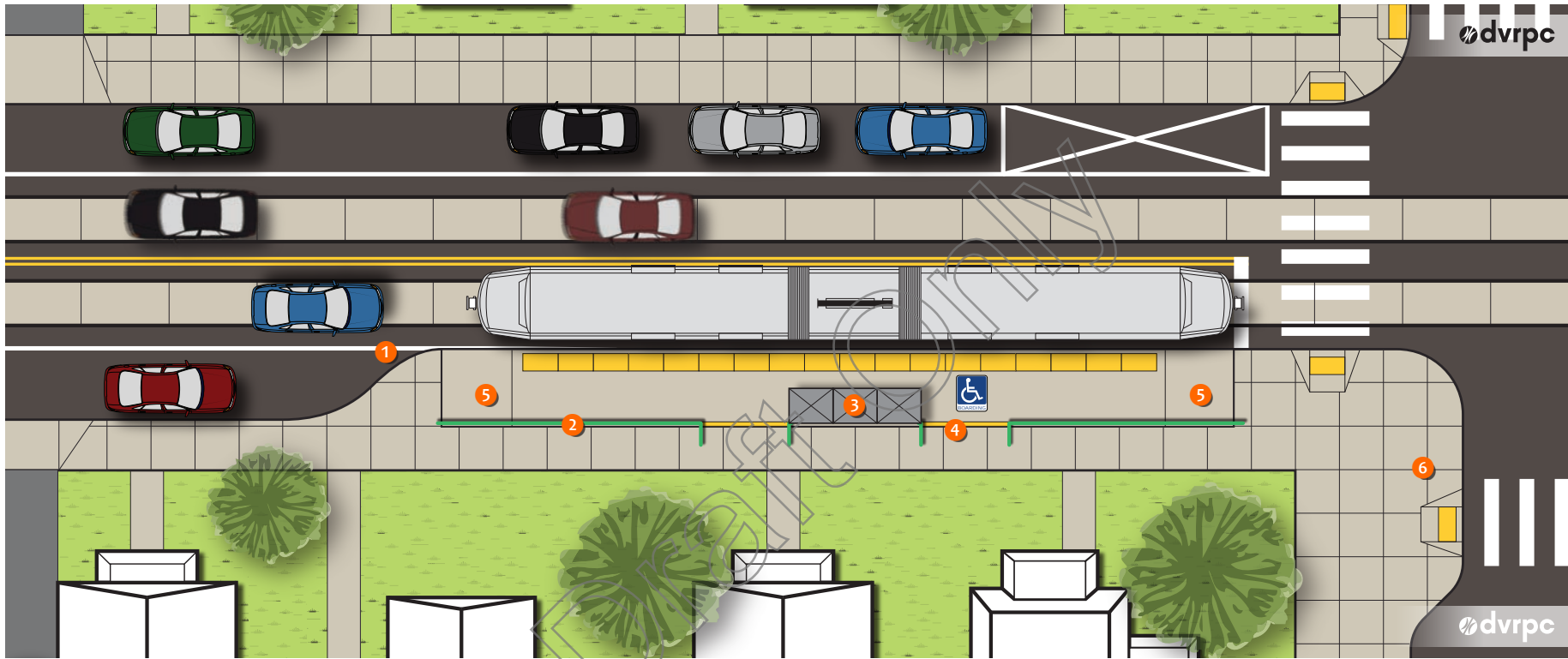
Figure 53 | Curb Extension Station: Plan
