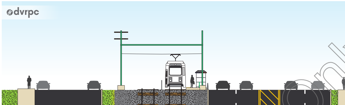
Figure 15 | Double track in exclusive right-of-way, typical cross-section
