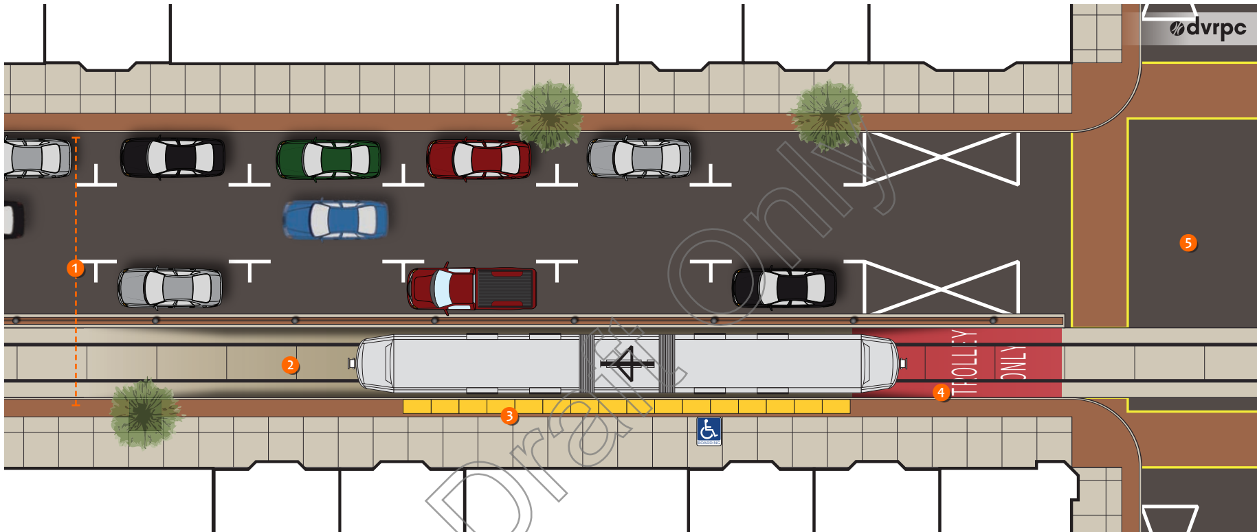
Figure 68 | One-way Street: Curbside Station: Plan
