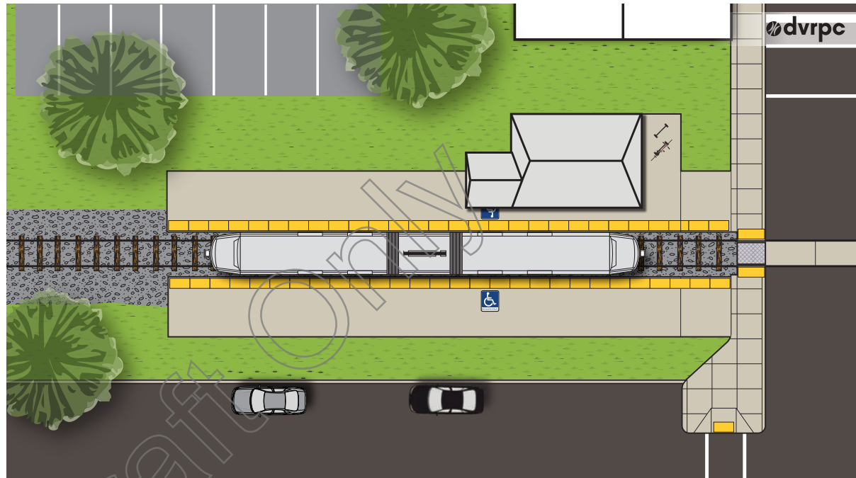
Figure 49 | Off-street Station: Single-track variation
